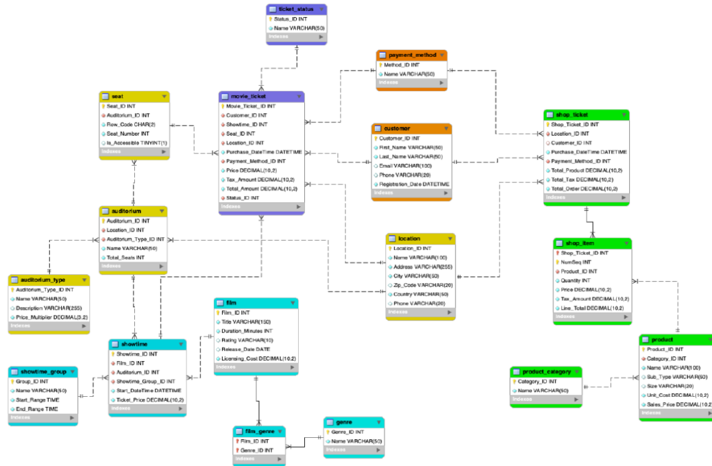
Figure 1. Entity–Relationship Diagram — Cinema Chain Database (MySQL Workbench)
